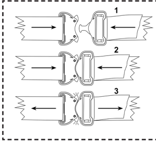
3.2a Manual (classic) buckles
