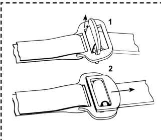
3.3a Fit the harness
